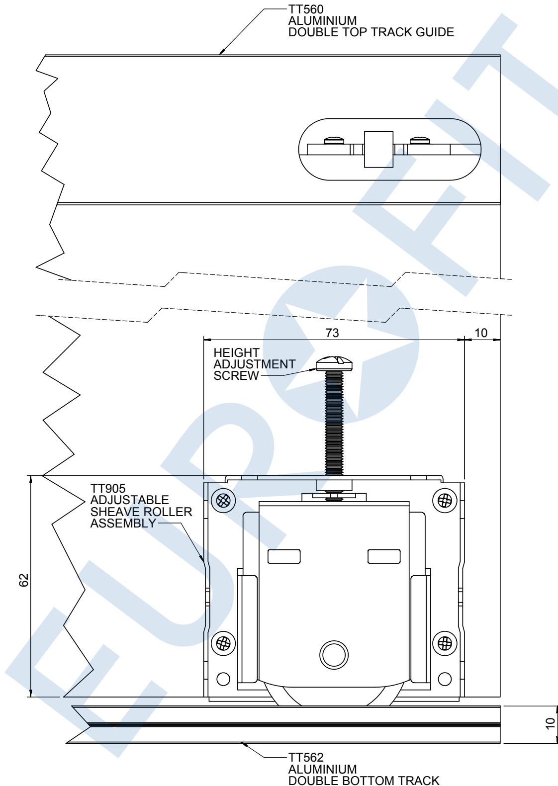
BACK VIEW BOTTOM MOUNTED DOUBLE DOOR
