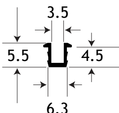
Sliding Door Lower Track
