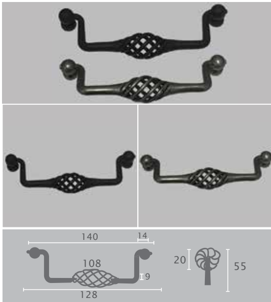
H148 Antique Bird Nest Swivel Handle
